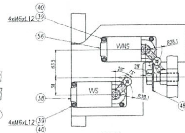
VIEW B
