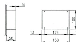
NAME PLATE BRACKET DETAIL
