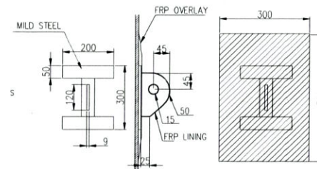
LIFTING LUGS DETAILS MATERIAL: MILD STEEL FRP LAMINATED 2 NOS. AT 120°, 300°
