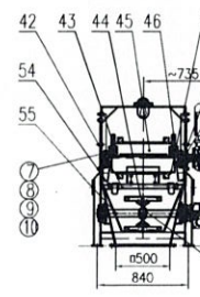
B-B Local view
