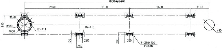
D-D Local view
