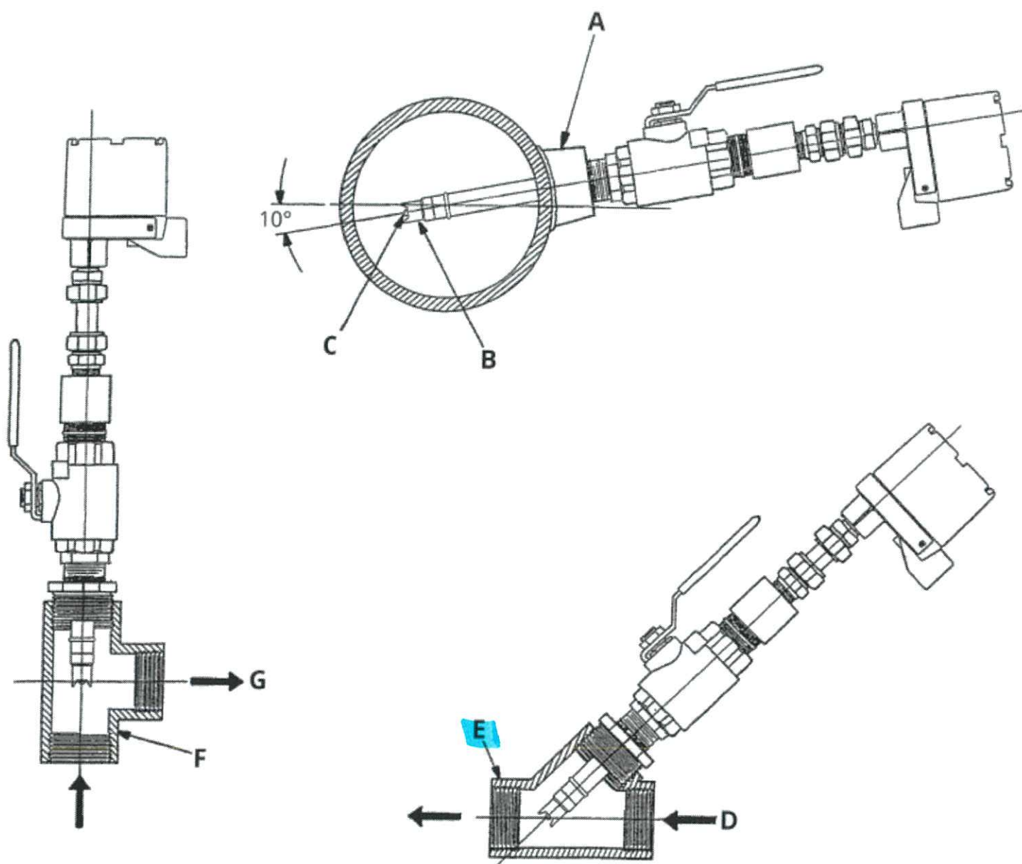
Figure 2-7: Typical Mounting Details for the Retractable Body Type Sensor (547)
