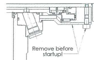
Seal with mounting spacers option
