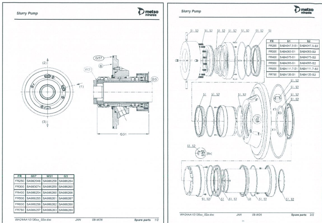
Metso Mechanical Seal Drawing (Based on O&M Manual)
