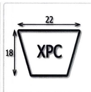
SPC belt dimension
