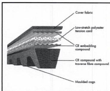
XPB belt profile
