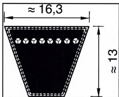
XPB/SPB belt dimension
