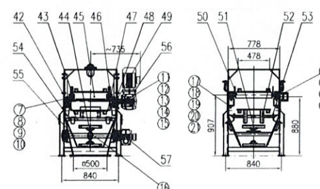
C-C Local view
