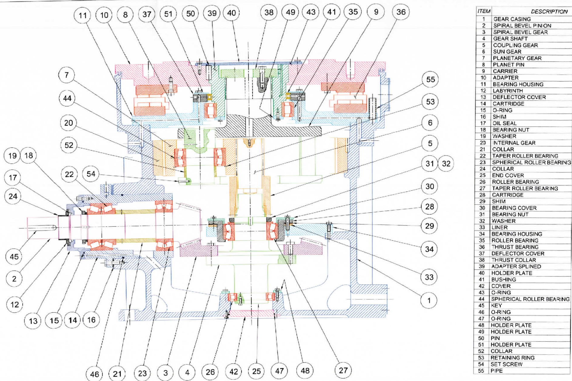
FIGURE 5-2 SECTIONAL VIEW OF PLANETARY GEARBOX
