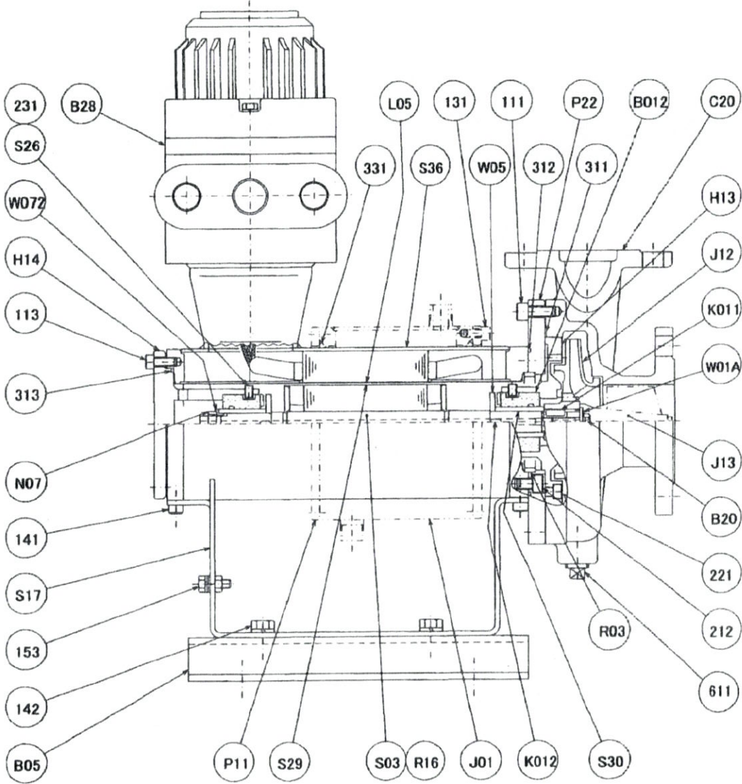
Fig. 1-1 HN Type (Basic Horizontal type) NON-SEAL PUMP
