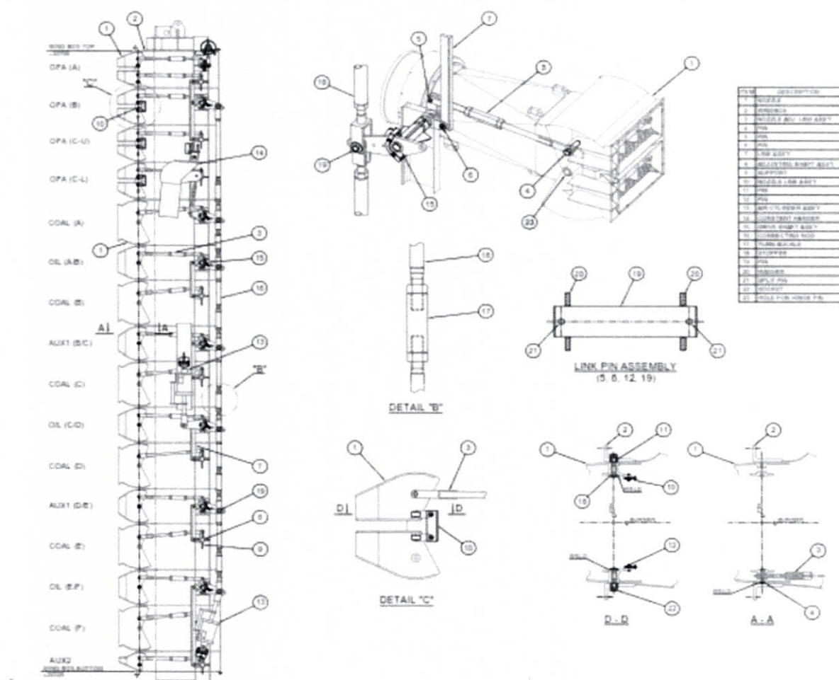
FIGURE 2-12 BURNER NOZZLE ANGLE ADJUSTING MECHANISM ARRANGEMENT
