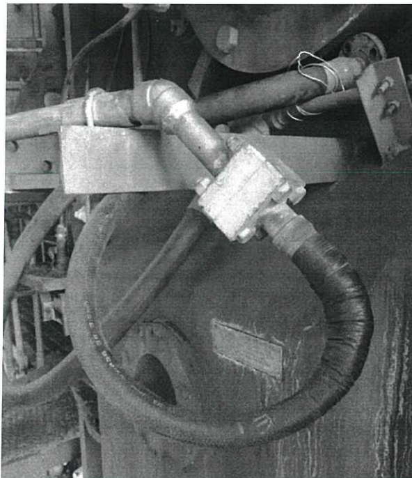
Hydraulic Line Current Condition (Rigid and Crack)
