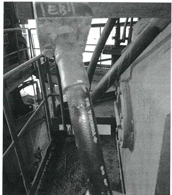
Hydraulic Line Current Condition (Rigid and Crack)
