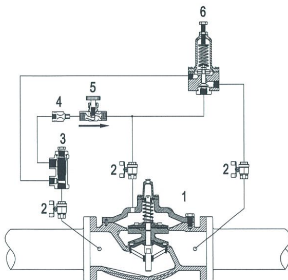
Schematic A-8700A
