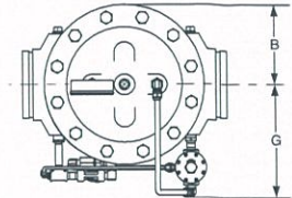
Model 50B-4KG1 Globe
