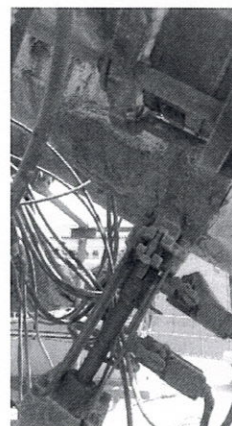
Leakage valve body due to ash abrasion
