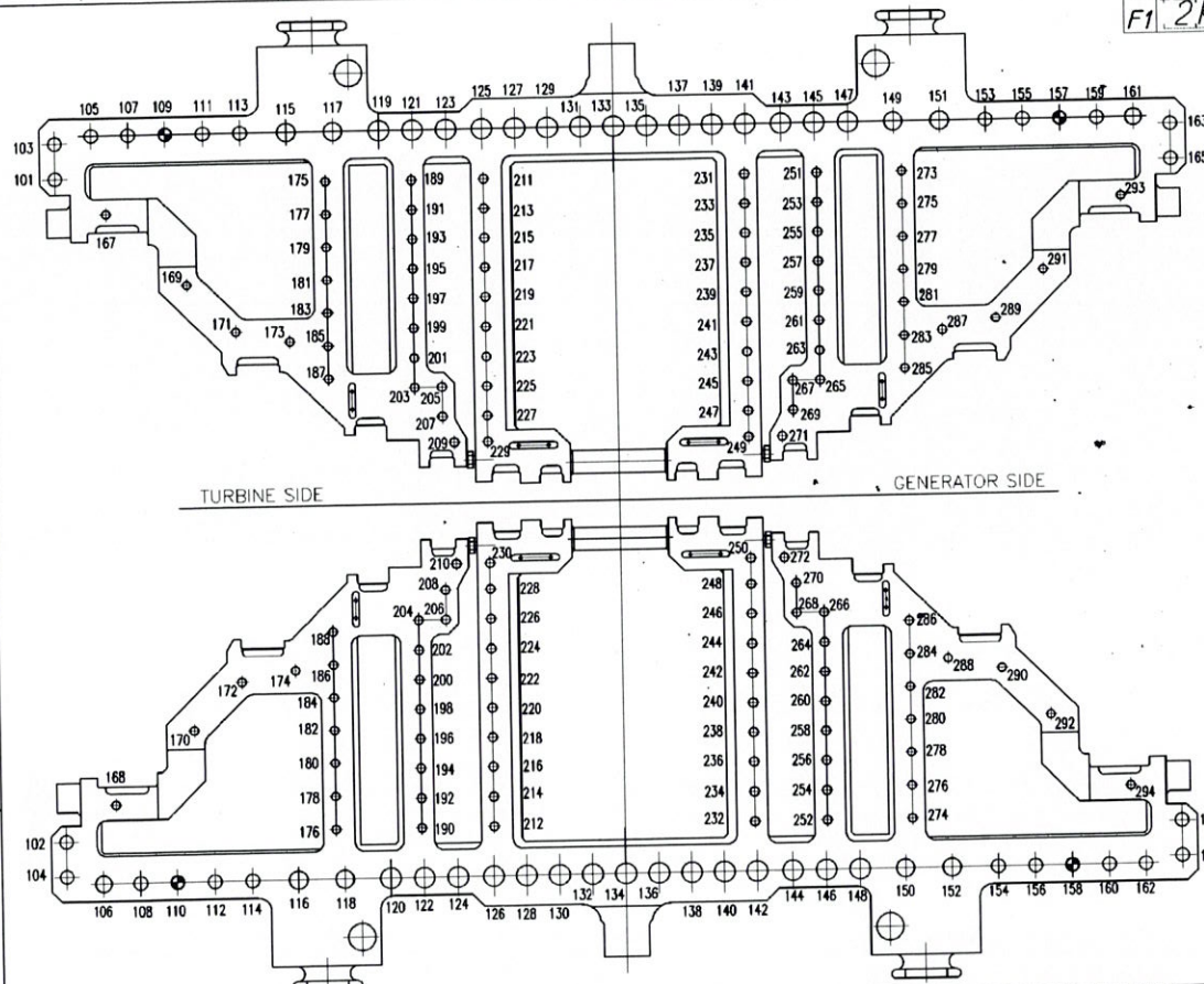
③① CROSSOVER PIPE FLANGE
