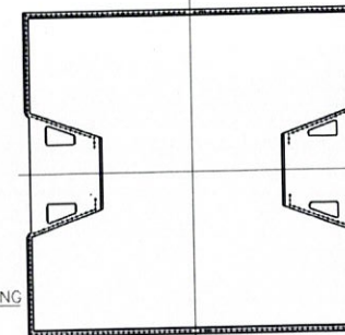
④ LP OUTER CASING HORIZONTAL STUD TOTAL 272 PIECE
