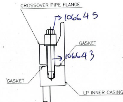
③① CROSSOVER PIPE FLANGE
