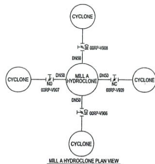
MILL A HYDROCLONE PLAN VIEW
