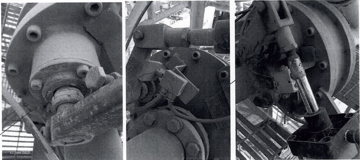
U4 RDDV current condition (ash leak from shaft assembly)
