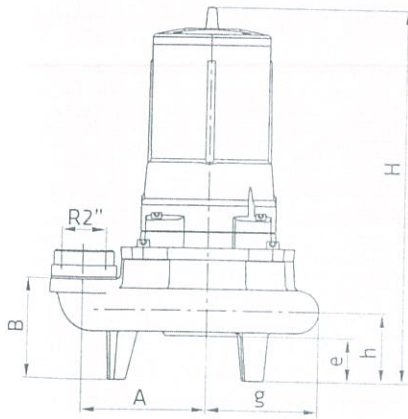
C 50 Hose Connection
