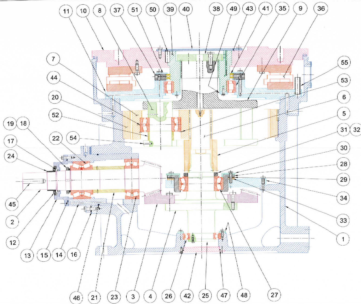
FIGURE 5-2 SECTIONAL VIEW OF PLANETARY GEARBOX
