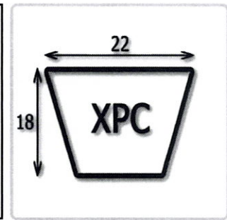
SPC belt dimension
