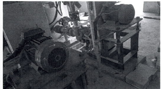
Limestone slurry feed & storage pumps
