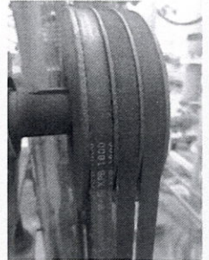
XPB belt profile
