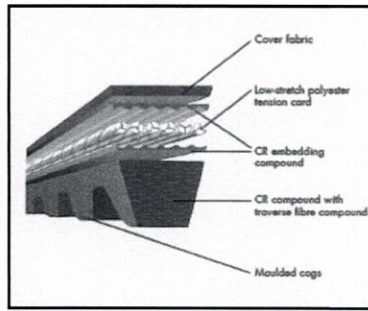
XPB belt profile
