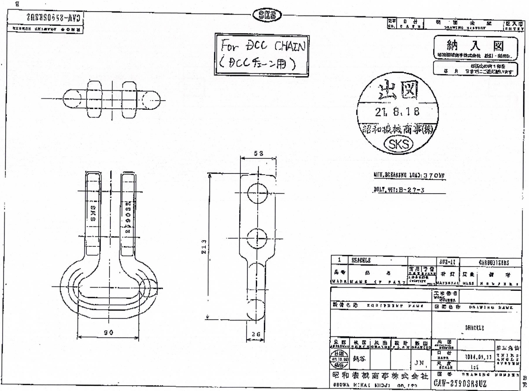
FIGURE E-7 SHACKLE
