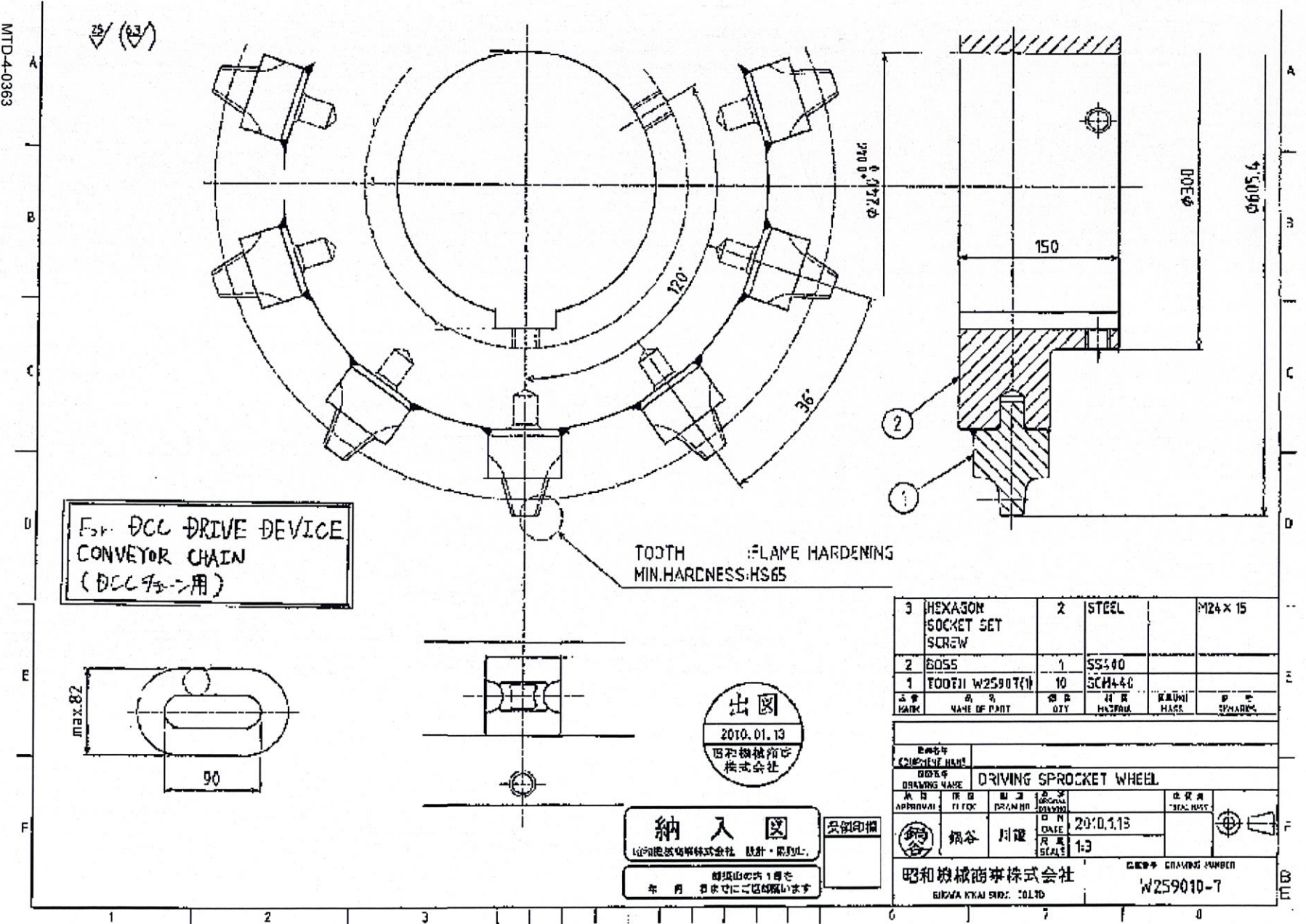
FIGURE E-5 DRIVING SPROCKET WHEEL
