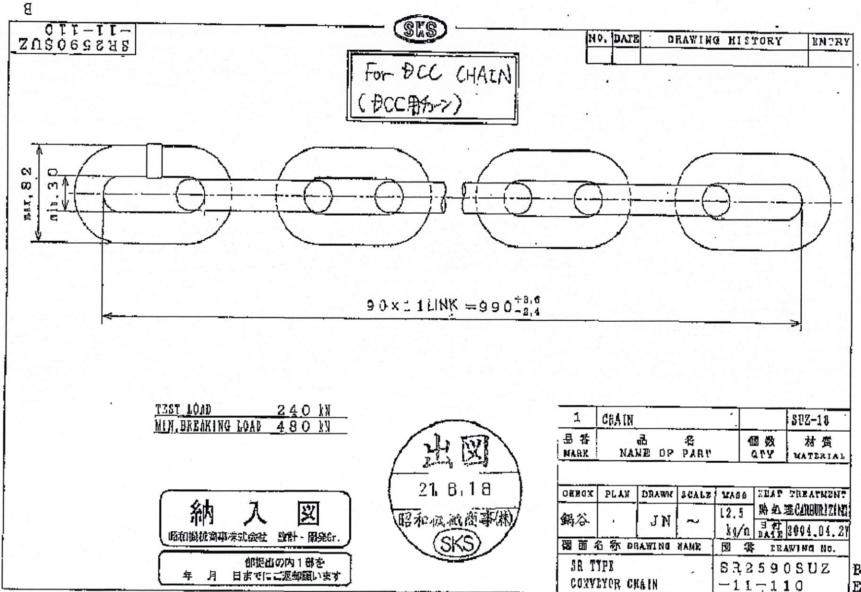
FIGURE E-6 CONVEYOR CHAIN
