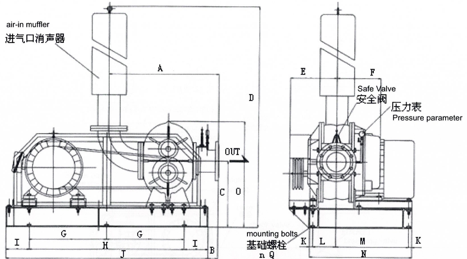
Outline dimensions for Model BK6008
