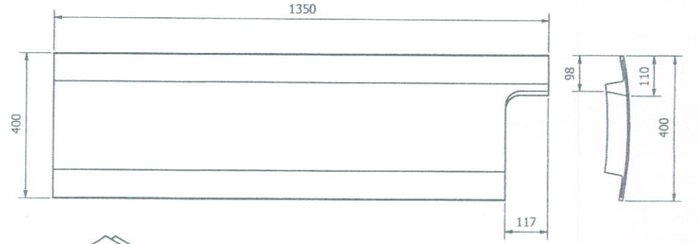
SHELL LINNER SL-C3
