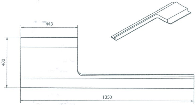
SHELL LINNER SL-C6
