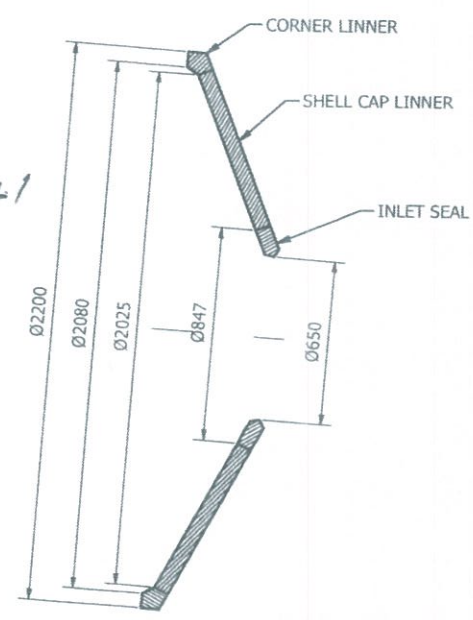
SECTION J-J
