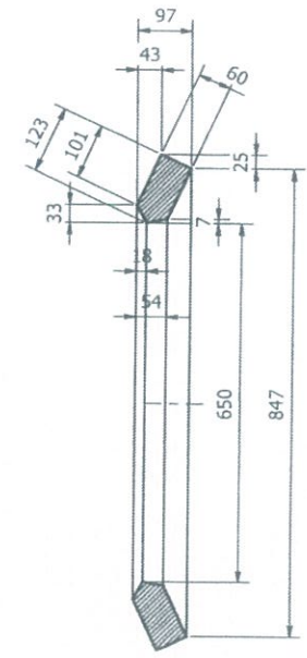
SECTION P-P
