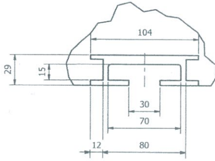
A (0.40 : 1)
