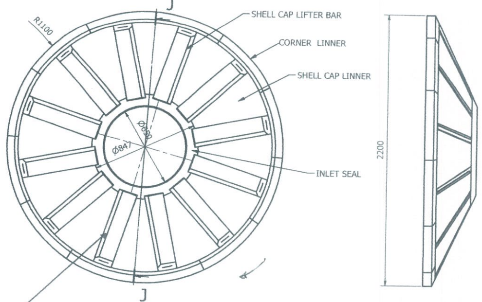
CAP SHELL LAYOUT
