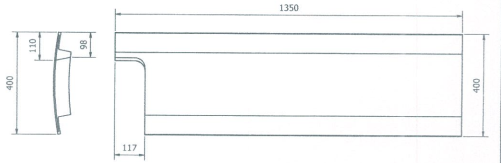
SHELL LINNER SL-C4
