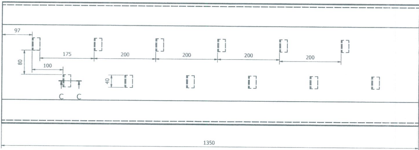
SHELL LINNER
