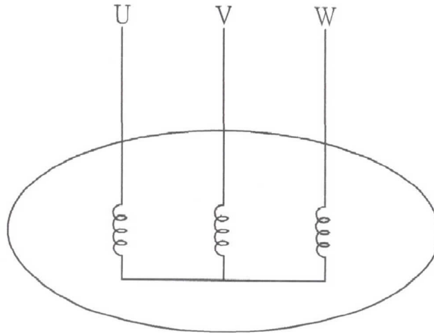
SCHEMATIC - WYE CONN - 3 LEADS
