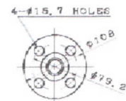
VIEW FROM A WATER INLET AND OUTLET, 1.00" NOM. ANSI B16.5 150LB FLANGE (ENLARGED VIEW)
