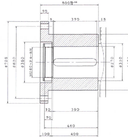
SHAFT END DETAIL ASSY (ENLARGED VIEW)
