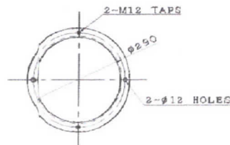
COUPLING NUT (ENLARGED VIEW)
