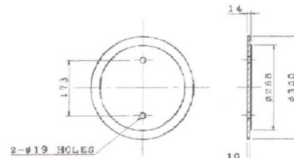
COUPLING NUT PLATE (ENLARGED VIEW)
