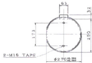
SHAFT END (ENLARGED VIEW)
