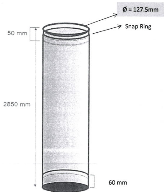
Drawing & Size of Bag Filter for Dust Collector
