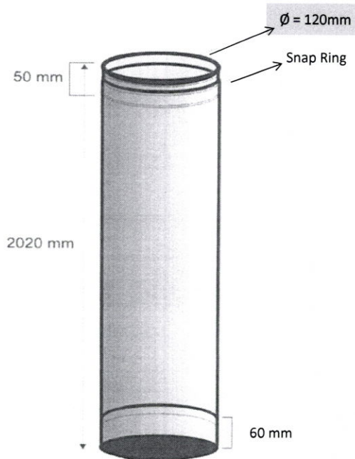
Drawing & Size of Bag Filter Fly Ash Silo
