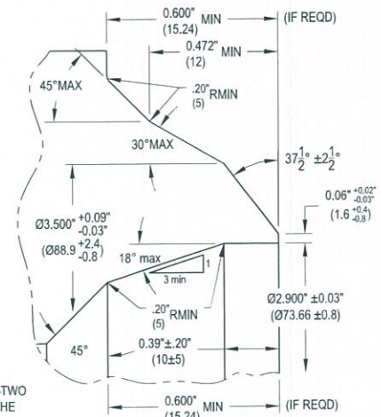
DETAIL 1B (OUTLET ONLY) BUTTWELD END MACHINING 3" SCH 80 t: 0.300" (7.62) AW1-80 x S8
