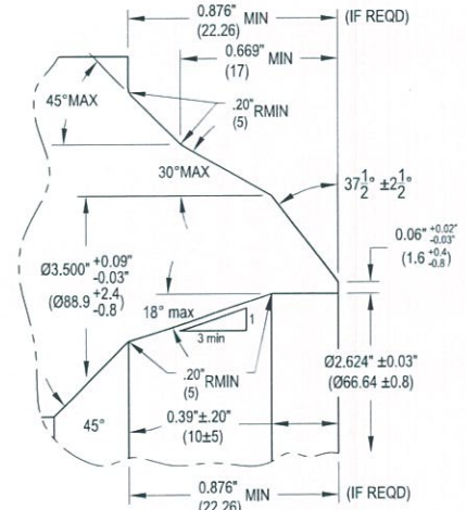
DETAIL 1A (INLET ONLY) BUTTWELD END MACHINING 3" SCH 160 t: 0.438" (11.13) AW1-80 x S16
