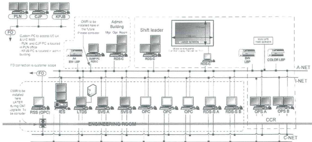
HMI LAYOUT COMMON
