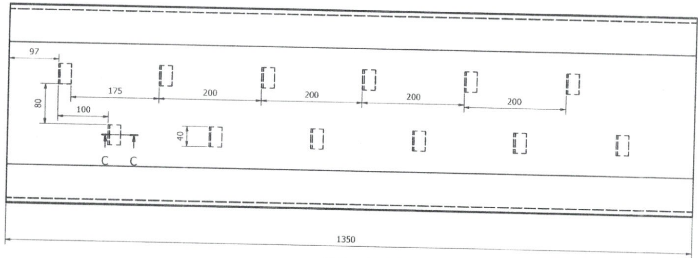
SHELL LINNER
