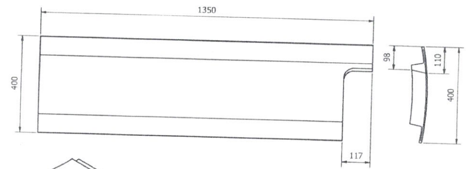
SHELL LINNER SL-C3
