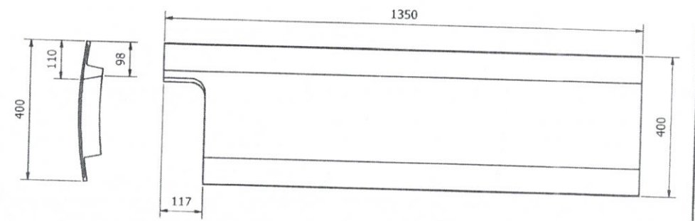
SHELL LINNER SL-C4
