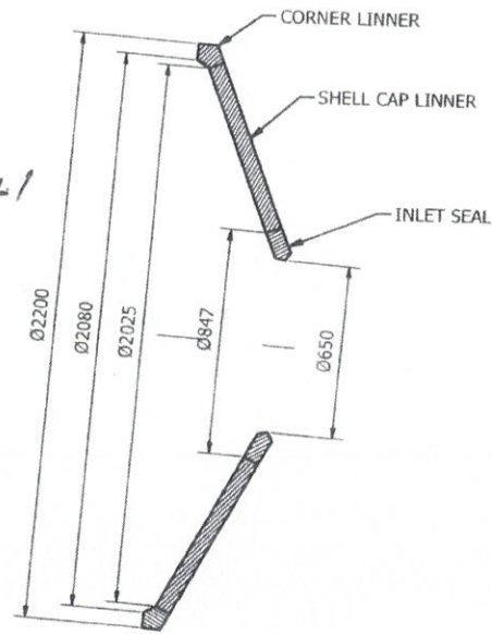
SECTION J-J
