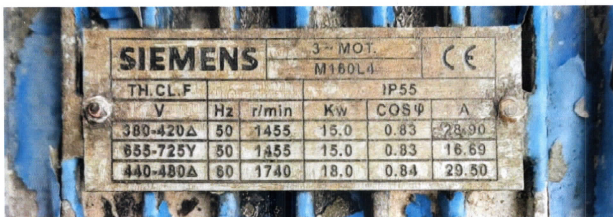
Motor Nameplate
