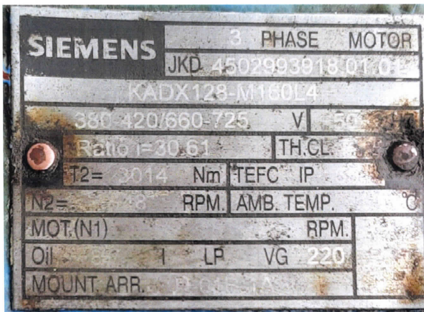
Gearbox Nameplate
