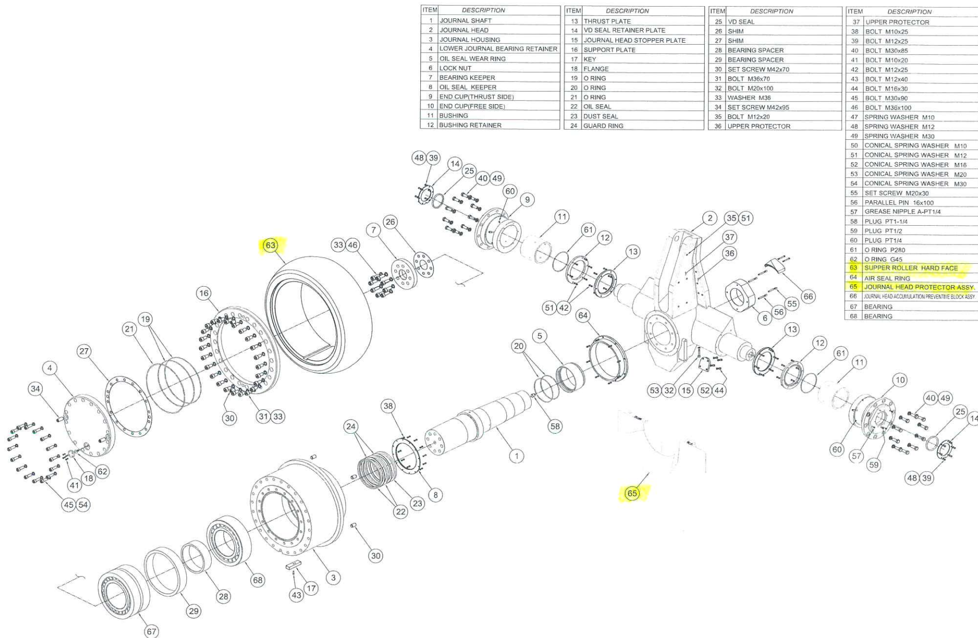
FIGURE 5-6 EXPLODED VIEW OF GRINDING ROLLER ASSEMBLY
