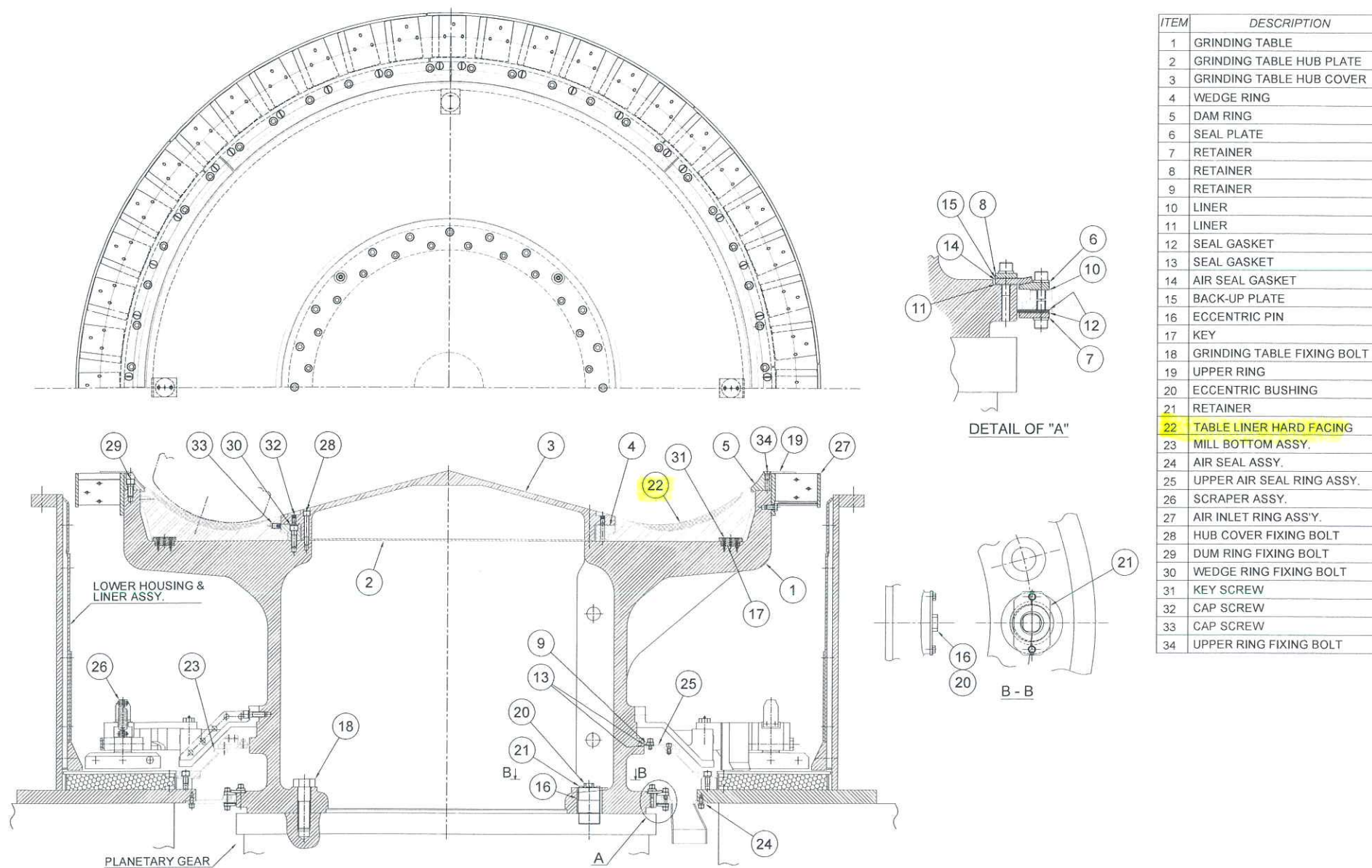
FIGURE 5-3 SECTIONAL VIEW OF GRINDING TABLE
